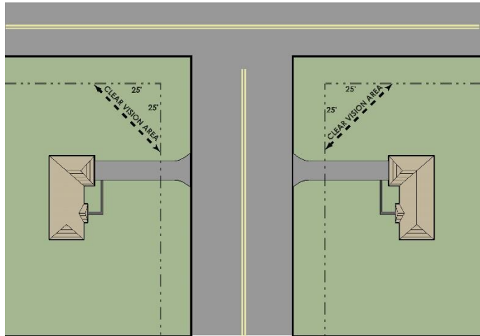
Figure 12-3: Clear vision corner
