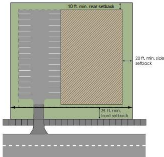
Figure 7-3: C-3 dimensional requirements
