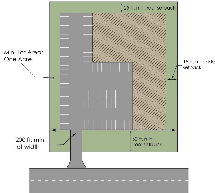
Figure 8-1: I-1 dimensional requirements
