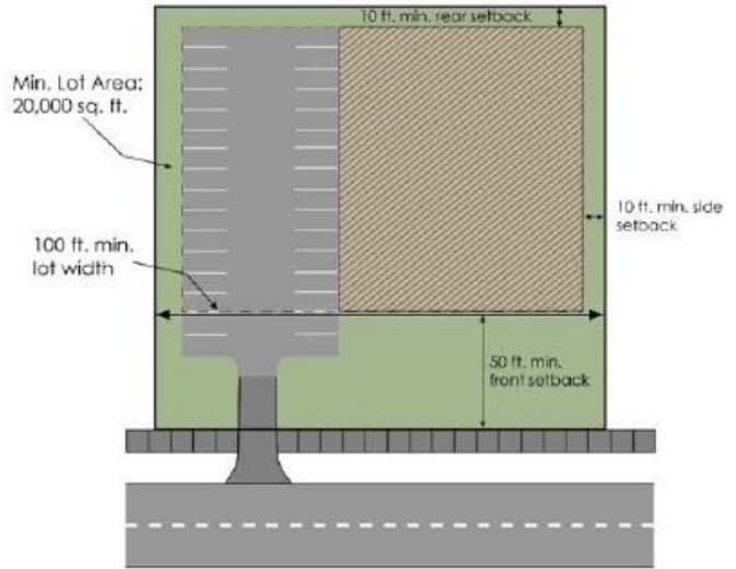
Figure 7-2: C-2 dimensional requirements
